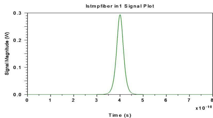
Fig.14: Input signal in time domain (N=3)
