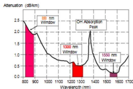
Fig.2. Optical fiber windows
