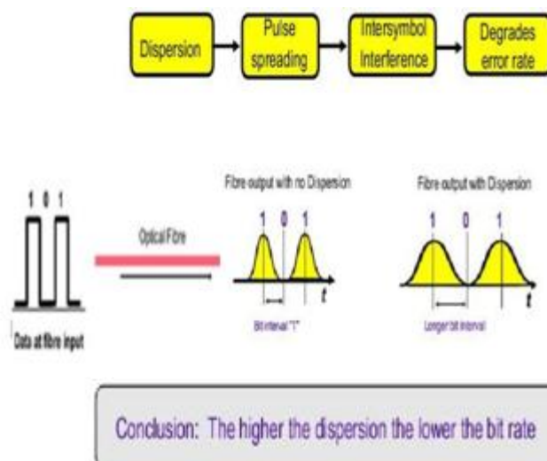
Fig.3: Dispersion in optical fiber
