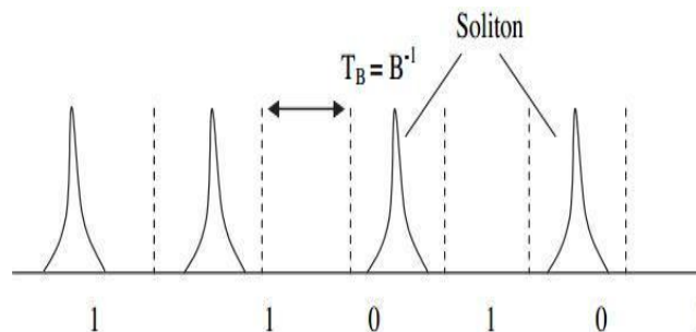
Fig.5. Soliton bit stream in an RZ format
